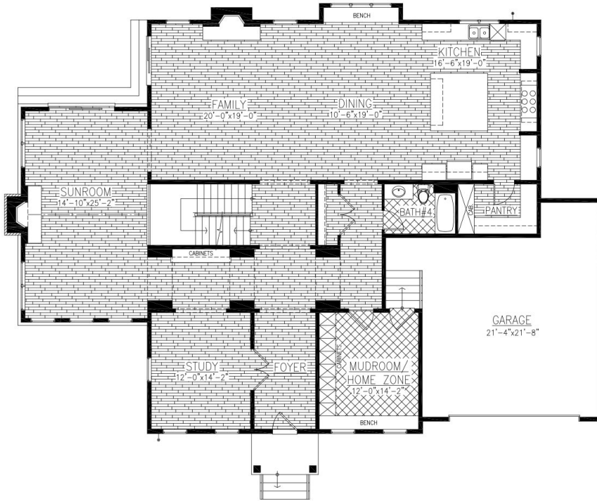
First Floor Plan Drawing
